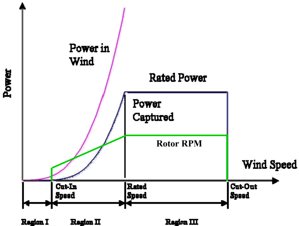
FIGURE 8. A typical power output versus wind speed curve.
