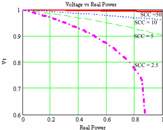
Figure 6. Terminal voltage as a function of real power for a VSWTG operated at \text{PF} = 0.95 under-excited
