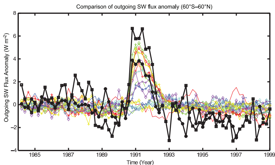
Figure 9.3. Comparison of outgoing shortwave radiation flux anomalies (in \text{W m}^{-2} , calculated relative to the entire time period) from several models in the MMD archive at PCMDI (coloured curves) with ERBS satellite data (black with stars; Wong et al., 2006) and with the ISCCP flux data set (black with squares; Zhang et al., 2004). Models shown are CCSM3, CGCM3.1(T47), CGCM3.1(T63), CNRM-CM3, CSIRO-MK3.0, FGOALS-g1.0, GFDL-CM2.0, GFDL-CM2.1, GISS-AOM, GISS-EH, GISS-ER, INM-CM3.0, IPSL-CM4, and MRI-CGCM2.3.2 (see Table 8.1 for model details). The comparison is restricted to 60^\circ\text{S} to 60^\circ\text{N} because the ERBS data are considered more accurate in this region. Note that not all models included the volcanic forcing from Mt. Pinatubo (1991–1993) and so do not predict the observed increase in outgoing solar radiation. See Supplementary Material, Appendix 9.C for additional information.
