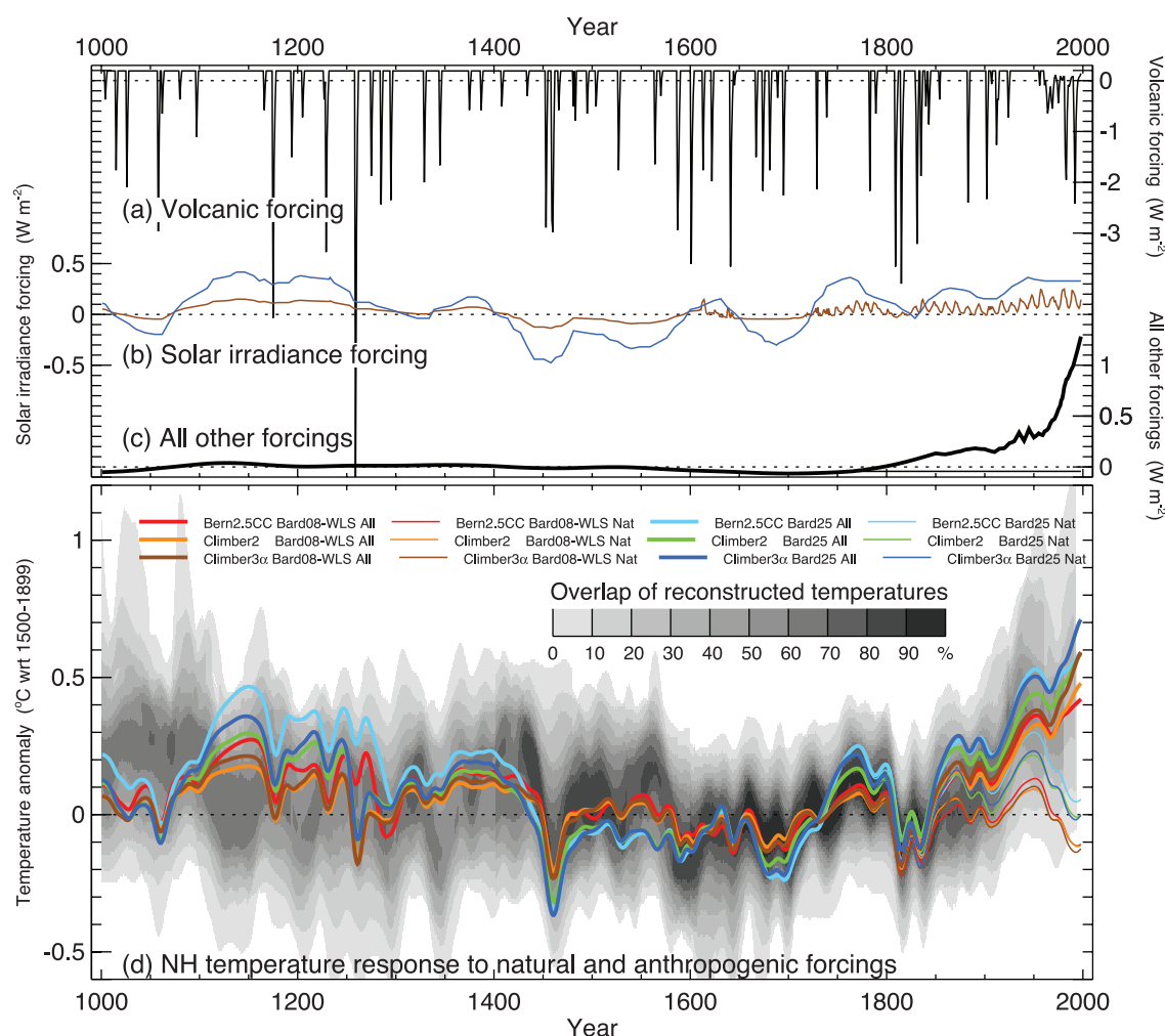
Figure 6.14. Simulated temperatures during the last 1 kyr with and without anthropogenic forcing, and also with weak or strong solar irradiance variations. Global mean radiative forcing ( \text{W m}^{-2} ) used to drive climate model simulations due to (a) volcanic activity, (b) strong (blue) and weak (brown) solar irradiance variations, and (c) all other forcings, including greenhouse gases and tropospheric sulphate aerosols (the thin flat line after 1765 indicates the fixed anthropogenic forcing used in the 'Nat' simulations). (d) Annual mean NH temperature ( ^{\circ}\text{C} ) simulated by three climate models under the forcings shown in (a) to (c), compared with the concentration of overlapping NH temperature reconstructions (shown by grey shading, modified from Figure 6.10c to account for the 1500 to 1899 reference period used here). 'All' (thick lines) used anthropogenic and natural forcings; 'Nat' (thin lines) used only natural forcings. All forcings and temperatures are expressed as anomalies from their 1500 to 1899 means; the temperatures were then smoothed with a Gaussian-weighted filter to remove fluctuations on time scales less than 30 years. Note the different vertical scale used for the volcanic forcing compared with the other forcings. The individual series are identified in Table 6.3.
