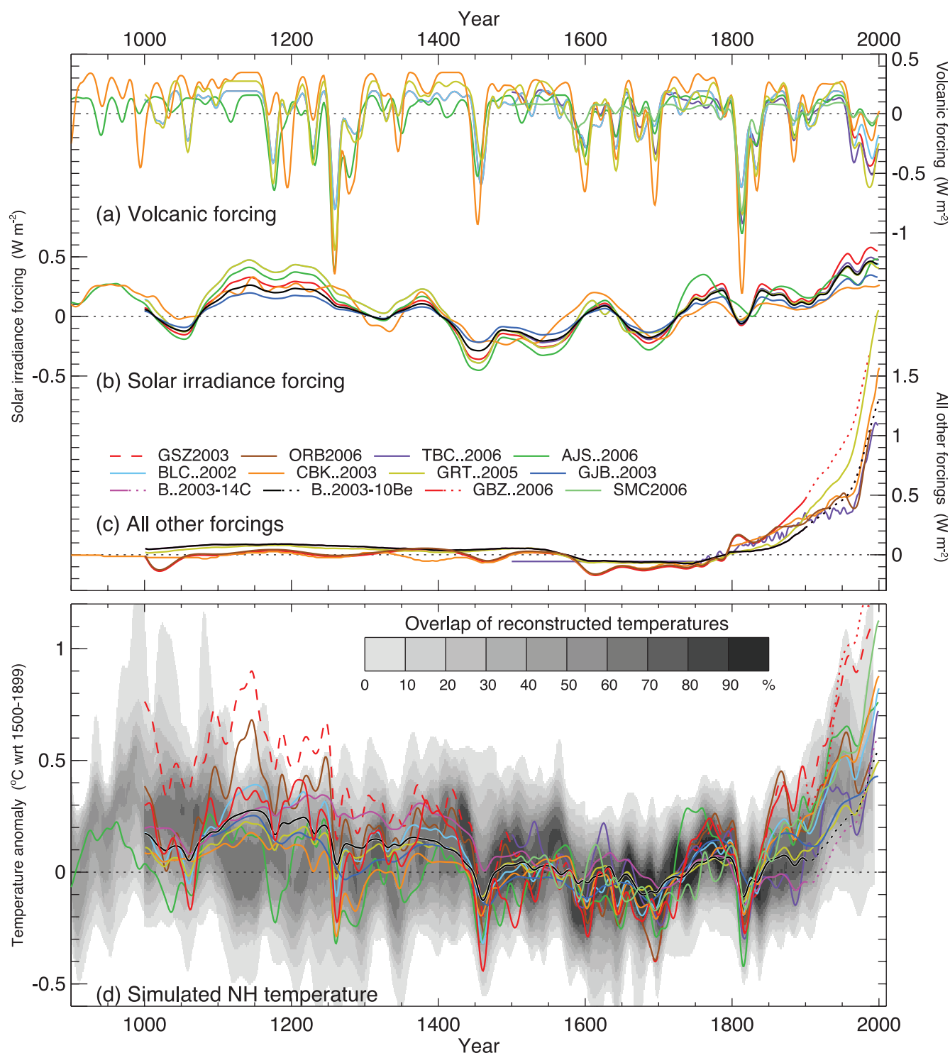
Figure 6.13. Radiative forcings and simulated temperatures during the last 1.1 kyr. Global mean radiative forcing ( \text{W m}^{-2} ) used to drive climate model simulations due to (a) volcanic activity, (b) solar irradiance variations and (c) all other forcings (which vary between models, but always include greenhouse gases, and, except for those with dotted lines after 1900, tropospheric sulphate aerosols). (d) Annual mean NH temperature ( ^{\circ}\text{C} ) simulated under the range of forcings shown in (a) to (c), compared with the concentration of overlapping NH temperature reconstructions (shown by grey shading, modified from Figure 6.10c to account for the 1500 to 1899 reference period used here). All forcings and temperatures are expressed as anomalies from their 1500 to 1899 means and then smoothed with a Gaussian-weighted filter to remove fluctuations on time scales less than 30 years; smoothed values are obtained up to both ends of each record by extending the records with the mean of the adjacent existing values. The individual series are identified in Table 6.2.
