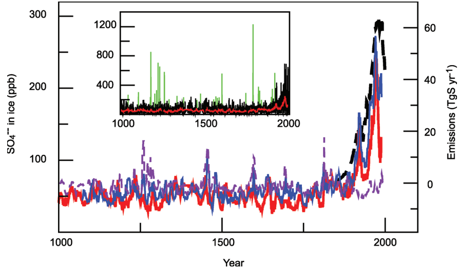
Figure 6.15. Sulphate ( \text{SO}_4^{2-} ) concentrations in Greenland (Bigler et al., 2002, red line; Mieding, 2005, blue) and antarctic (Traufetter et al., 2004, dash, violet) ice cores during the last millennium. Also shown are the estimated anthropogenic sulphur (S) emissions for the NH (Stern, 2005; dashed black). The ice core data have been smoothed with a 10-year running median filter, thereby removing the peaks of major volcanic eruptions. The inset illustrates the influence of volcanic emissions over the last millennium and shows monthly sulphate data in ppm as measured (green), with identified volcanic spikes removed (black, most recent volcanic events were not assigned nor removed), and results from the 10-year filter (red) (Bigler et al., 2002). The records represent illustrative examples and can be influenced by local deposition events.
