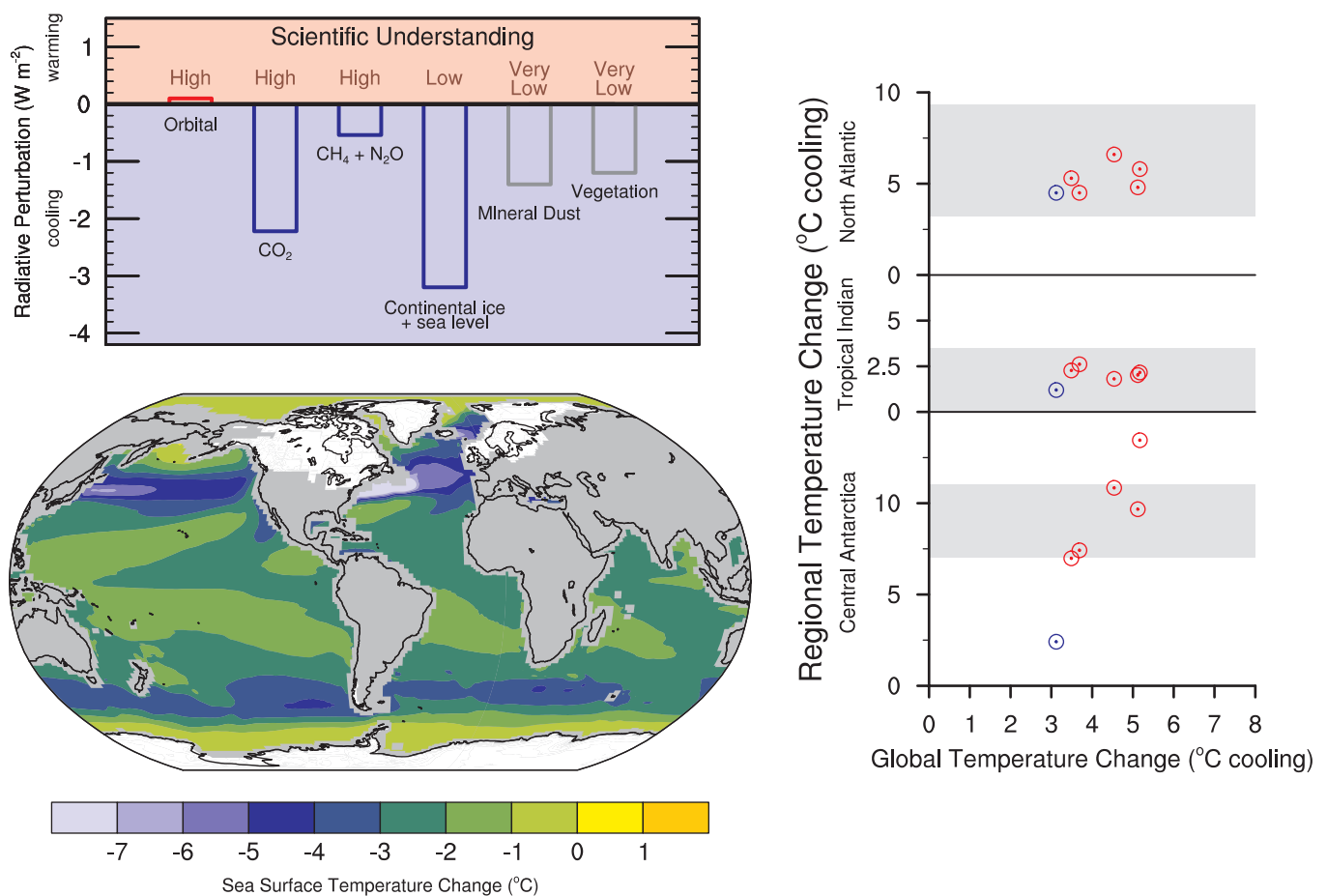
Figure 6.5. The Last Glacial Maximum climate (approximately 21 ka) relative to the pre-industrial (1750) climate. (Top left) Global annual mean radiative influences (W m -2 ) of LGM climate change agents, generally feedbacks in glacial-interglacial cycles, but also specified in most Atmosphere-Ocean General Circulation Model (AOGCM) simulations for the LGM. The heights of the rectangular bars denote best estimate values guided by published values of the climate change agents and conversion to radiative perturbations using simplified expressions for the greenhouse gas concentrations and model calculations for the ice sheets, vegetation and mineral dust. References are included in the text. A judgment of each estimate's reliability is given as a level of scientific understanding based on uncertainties in the climate change agents and physical understanding of their radiative effects. Paleoclimate Modelling Intercomparison Project 2 (PMIP-2) simulations shown in bottom left and right panels do not include the radiative influences of LGM changes in mineral dust or vegetation. (Bottom left) Multi-model average SST change for LGM PMIP-2 simulations by five AOGCMs (Community Climate System Model (CCSM), Flexible Global Ocean-Atmosphere-Land System (FGOALS), Hadley Centre Coupled Model (HadCM), Institut Pierre Simon Laplace Climate System Model (IPSL-CM), Model for Interdisciplinary Research on Climate (MIROC)). Ice extent over continents is shown in white. (Right) LGM regional cooling compared to LGM global cooling as simulated in PMIP-2, with AOGCM results shown as red circles and EMIC (ECBilt-CLIO) results shown as blue circles. Regional averages are defined as: Antarctica, annual for inland ice cores; tropical Indian Ocean, annual for 15°S to 15°N, 50°E to 100°E; and North Atlantic Ocean, July to September for 42°N to 57°N, 35°W to 20°E. Grey shading indicates the range of observed proxy estimates of regional cooling: Antarctica (Stenni et al., 2001; Masson-Delmotte et al., 2006), tropical Indian Ocean (Rosell-Mele et al., 2004; Barrows and Juggins, 2005), and North Atlantic Ocean (Rosell-Mele et al., 2004; Kucera et al., 2005; de Vernal et al., 2006; Kageyama et al., 2006).
