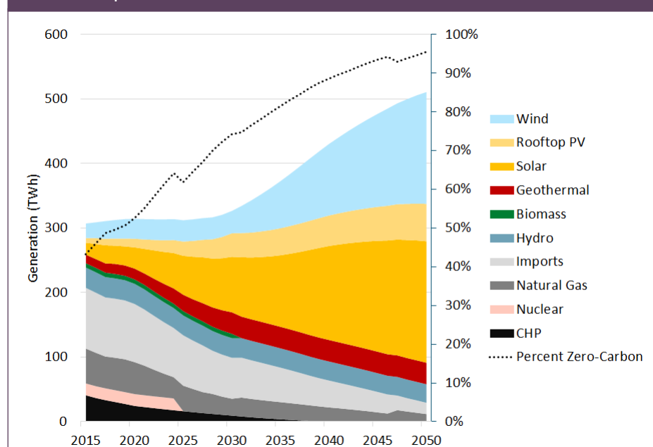
FIGURE 12 | PROJECTING TOTAL ELECTRICITY GENERATION THROUGH 2050
