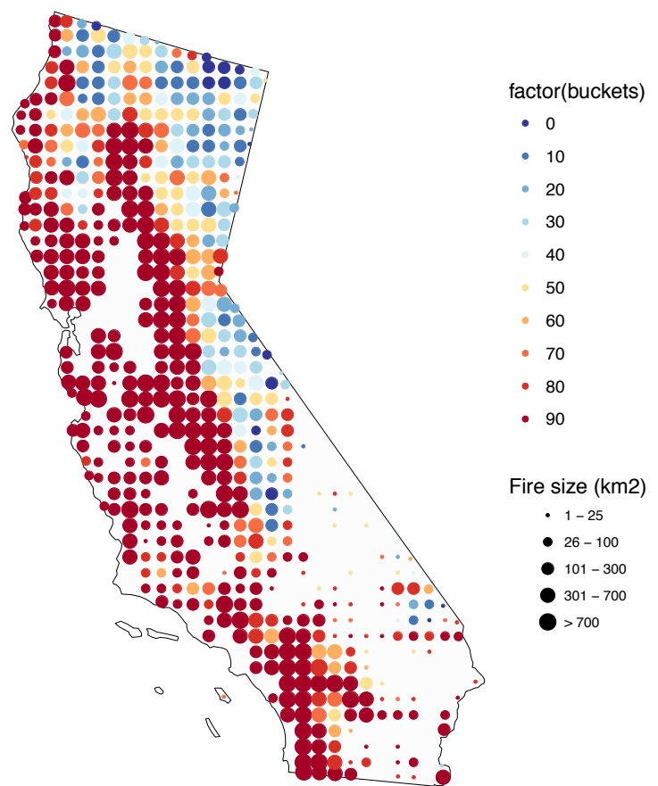
FIGURE 7 | WILDFIRES FROM 1992-2012
